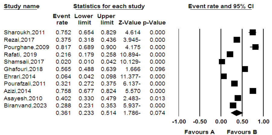
Meta Analysis
